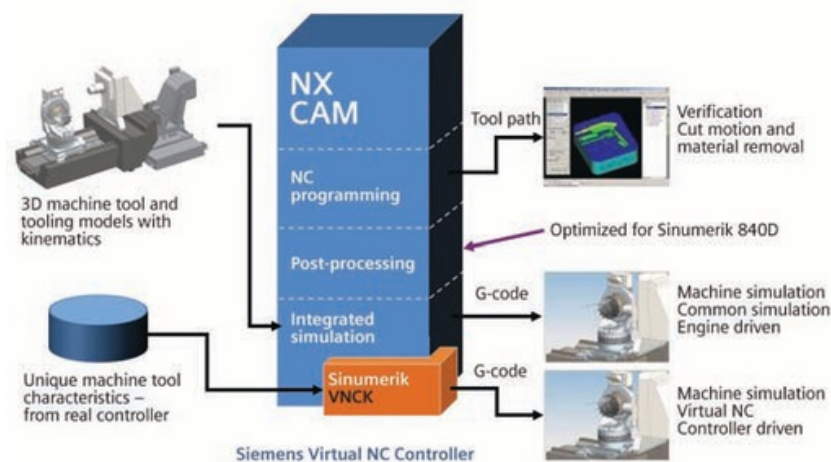
NX controller-driven machine tool simulation.
